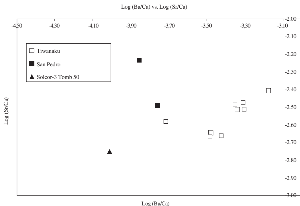
Figure 6. Trace element concentration data of modern and archaeological fauna from the San Pedro de Atacama oasis and the southeastern Lake Titicaca Basin where Tiwanaku is located, as well as trace element concentration data on a rib fragment from the adult male buried in Tomb 50.
